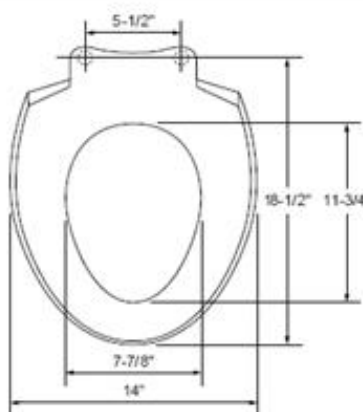
Model SS154 for Elongated Bowls
